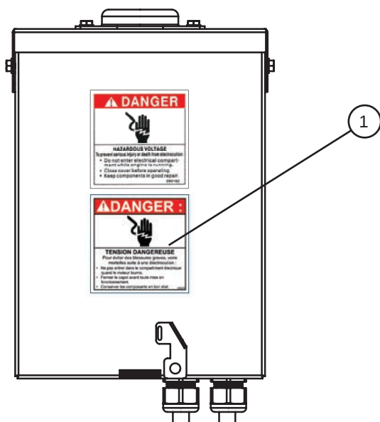
OUTSIDE OF BREAKER BOX
